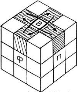
A4 \Phi T^{-1} B (P^2 B^2)^3 B^{-1} T \Phi^{-1} \begin{cases} \delta l \rightleftharpoons \delta n \\ \delta \phi \rightleftharpoons \delta t \end{cases}
